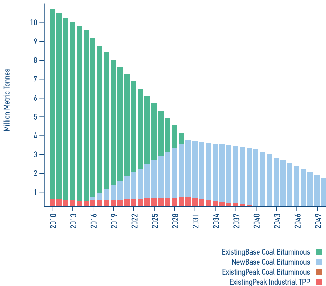
Chart 41: Carbon dioxide emission from the power sector in BiH according to the scenario S3 – advanced mitigation scenario
